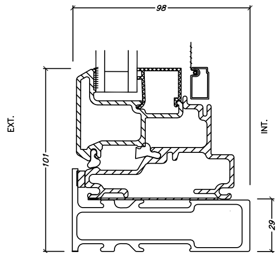
2a 400 Series with 325 Series Casement / Awning
